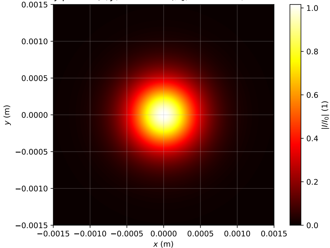
Intensity profile I(x, y, z = 3.344m)/I_0 , P_{in}=0.8P_{cr} , artificial time
